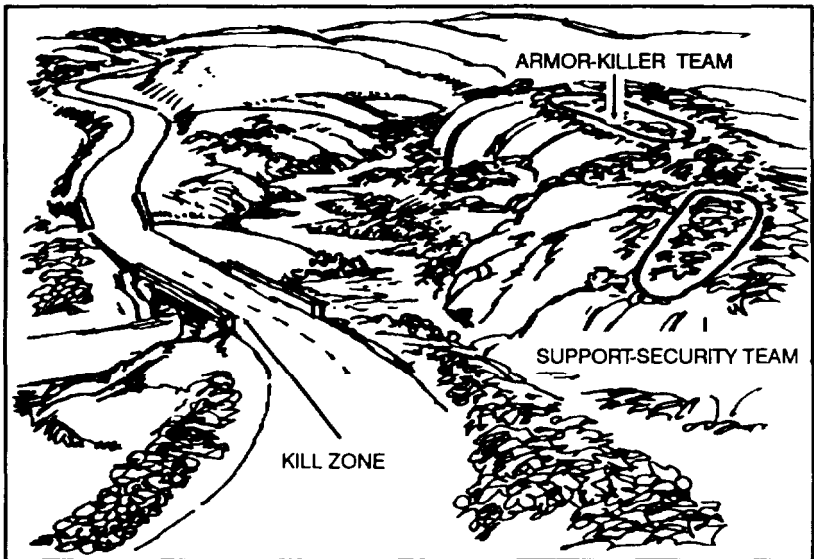
Figure 3-16. Antiarmor ambush.
